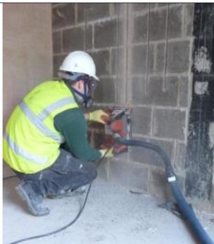
Good practice – Chasing concrete with on-tool extraction (HSE, GB)
